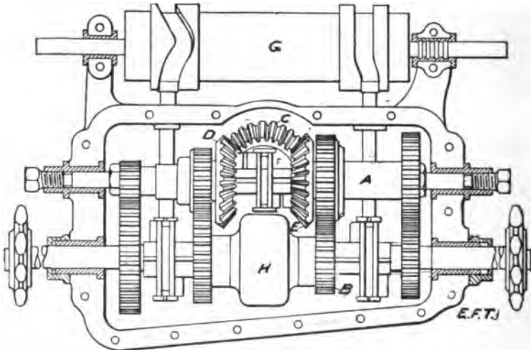
FIG. 351.—Details of the Montauban-Marchandier Change Speed Gear. A is the first motion shaft, to which are keyed four spurs of different diameters; B , the second motion shaft, carrying four loose spurs, capable of being engaged by clutches. C is a bevel on the drive shaft of the engine. D and E are bevels in mesh with C and capable of being tightened or loosened by the sliding shaft clutch, F , thus varying the direction of travel. G is a cam drum, by rotating which any desired spur on B may be clutched and thrown into gear with its mate on A .
